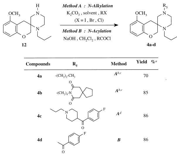
Scheme 5. a Yields of isolated products based on amine 12 , after purification by column chromatography. b For the synthesis of 4a and 4b see ref 54. c Acetone was the solvent. d Acetonitrile was used as solvent in the presence of a catalytic amount of potassium iodide.
