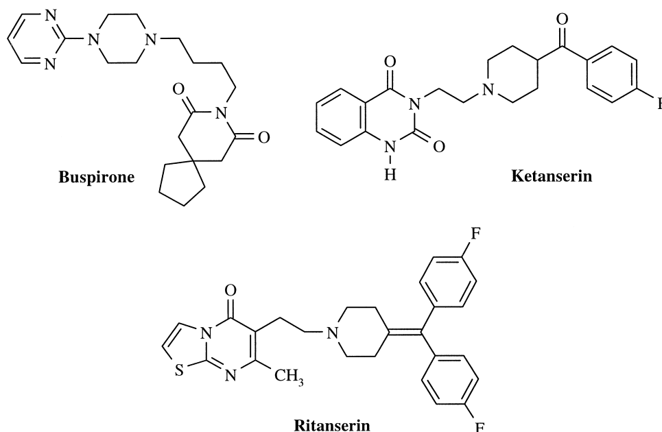
Figure 1. Structure of buspirone, ketanserin and ritanserin.
