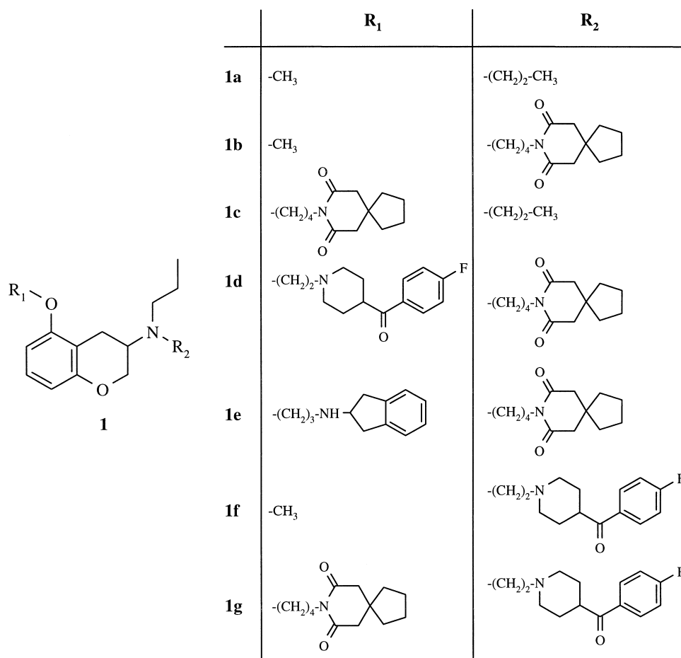
Figure 3. Structure of N -substituted-3-amino-5-alkoxy-3,4-dihydro-2 H -1-benzopyran derivatives 1 .
