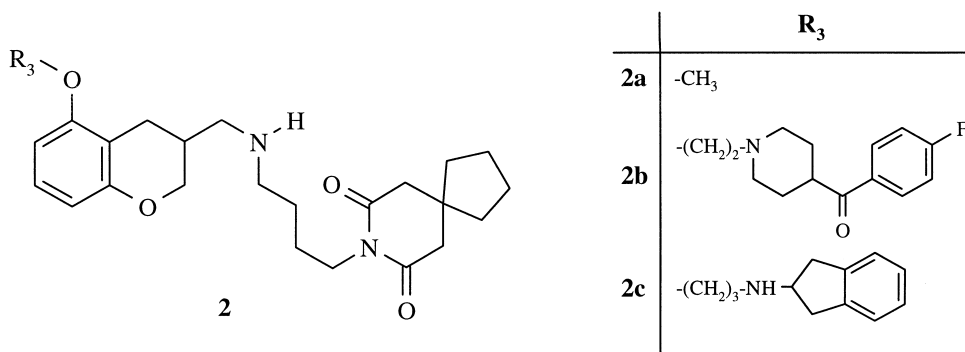
Figure 4. Structure of N -substituted-3-aminomethyl-5-alkoxy-3,4-dihydro-2 H -1-benzopyran derivatives 2 .
