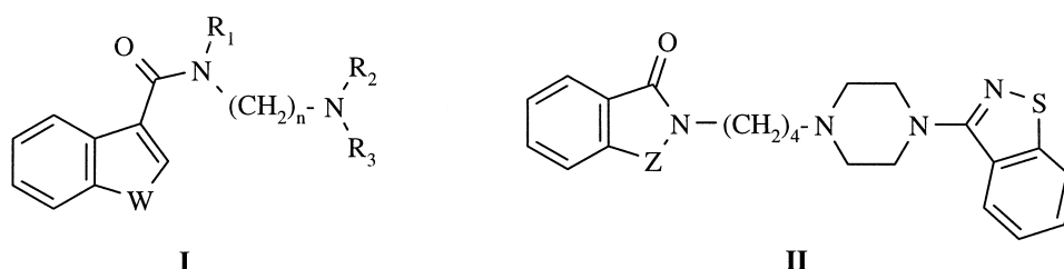
Figure 2. Structure of (1,2-benzisothiazole-3-yl) piperazine derivatives I and benzisothiazole-3-carboxamide derivatives II .
